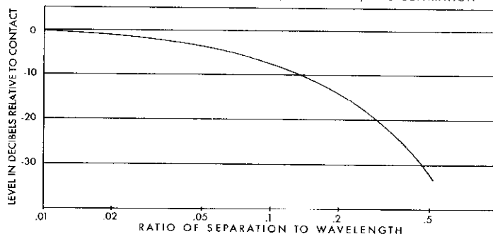
FIG. 2 SIGNAL ATTENUATION CAUSED BY POOR CONTACT IN PLAYBACK UNIVERSAL CURVE FOR ANY SPEED, FREQUENCY, AND SEPARATION
