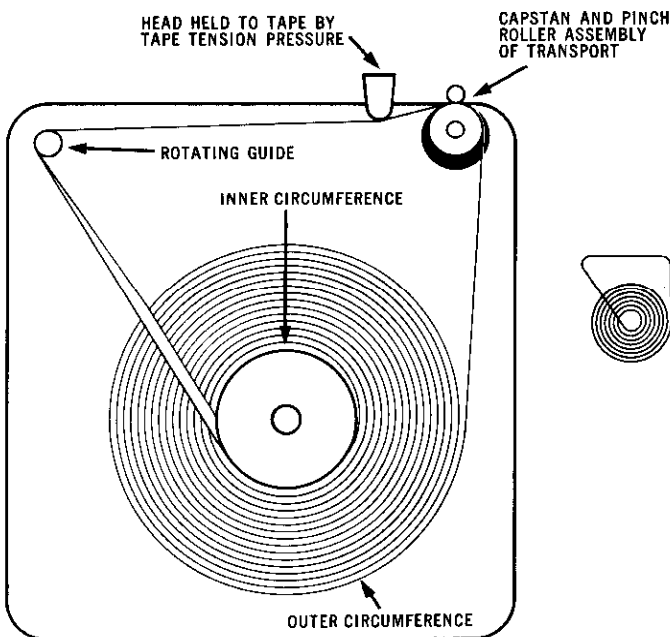
CONTINUOUS LOOP TAPE CARTRIDGE
