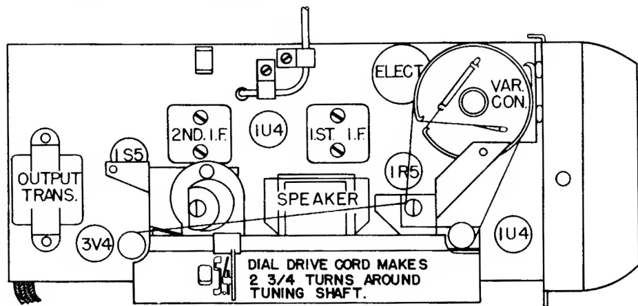
TUBE LAYOUT
