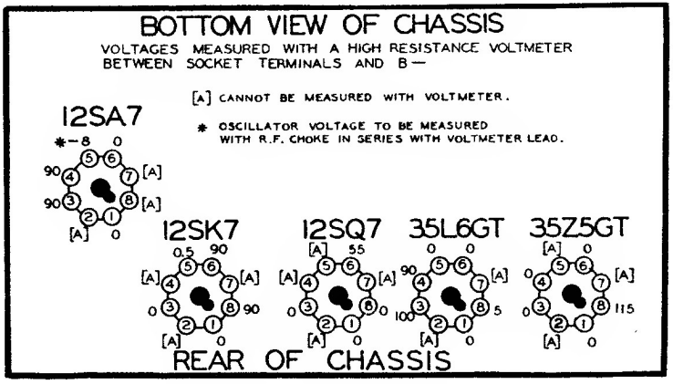
VIEW LOOKING AT BOTTOM OF CHASSIS
