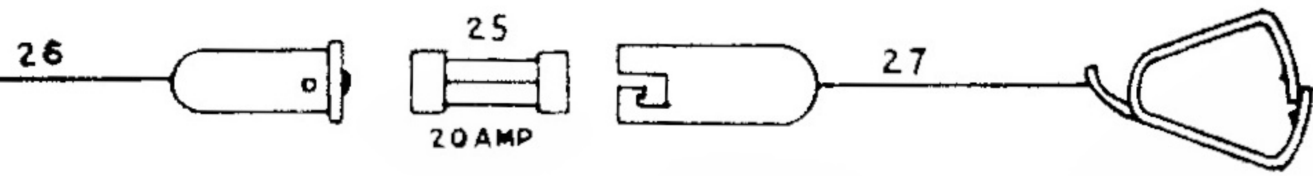
985-425 WIRING DIAGRAM
