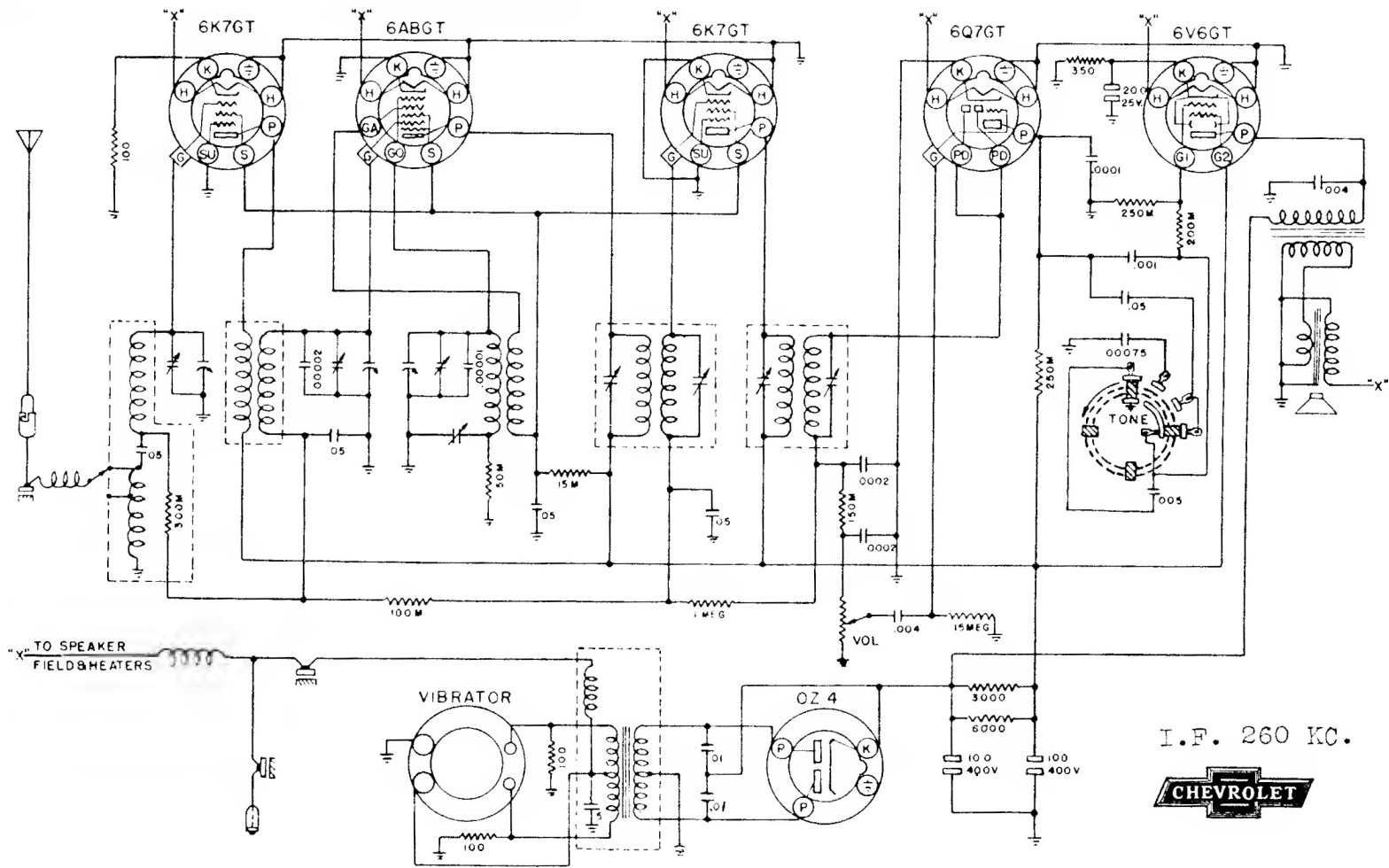
985537 CIRCUIT DIAGRAM
