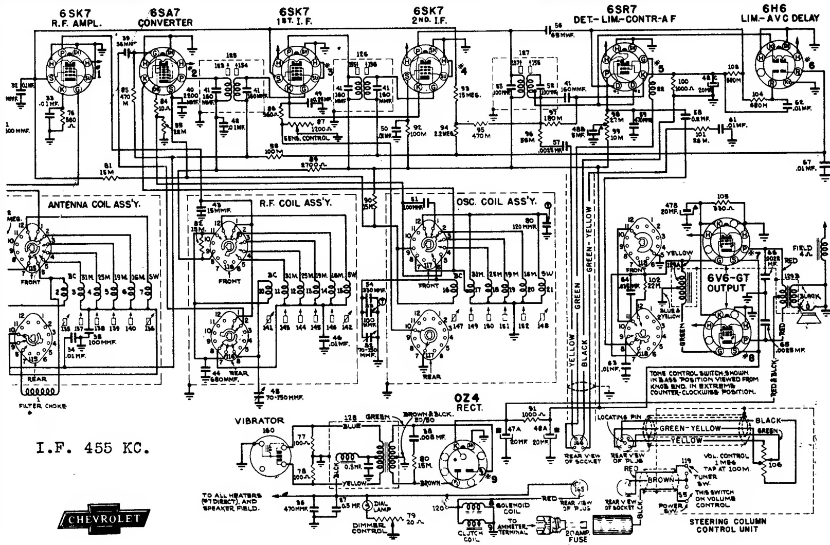
CIRCUIT DIAGRAM—RADIO 985794
