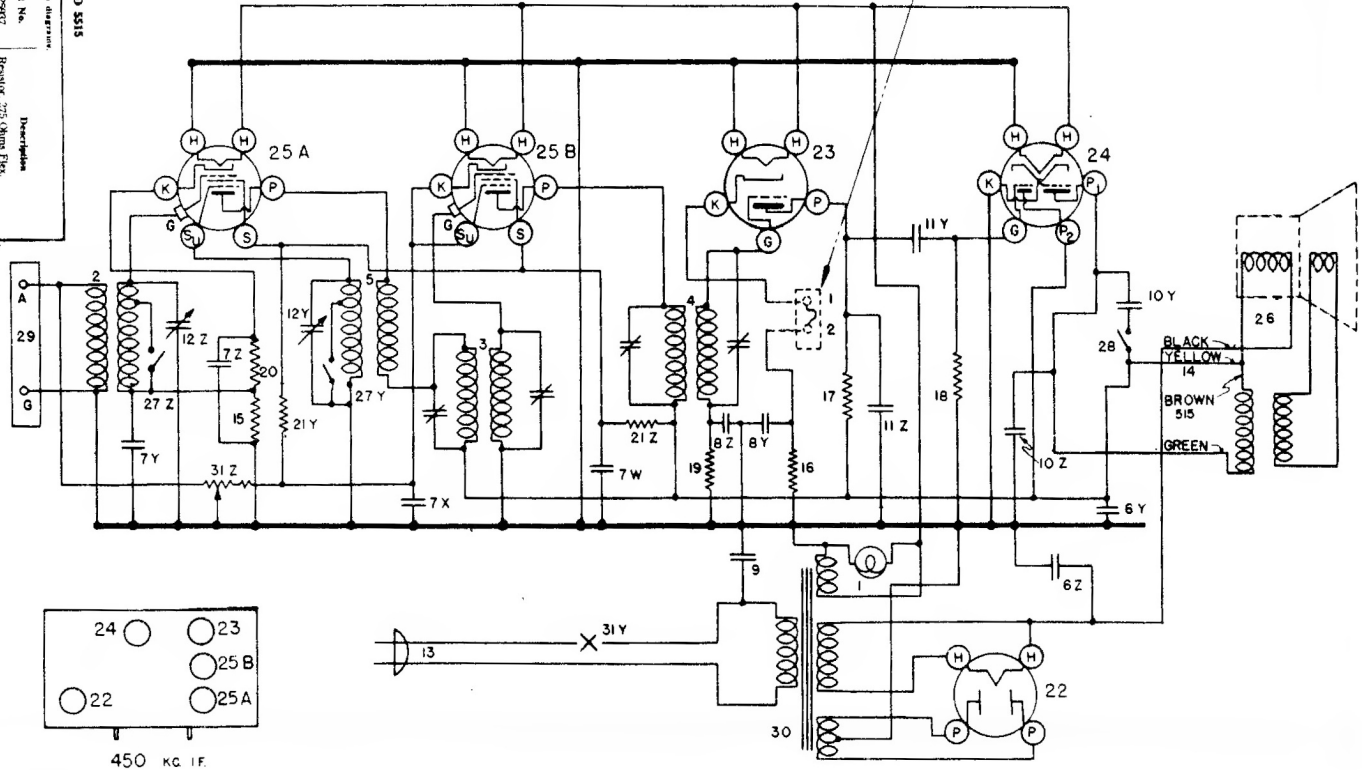
WIRING DIAGRAM OF MODELS 515 AND 5515
