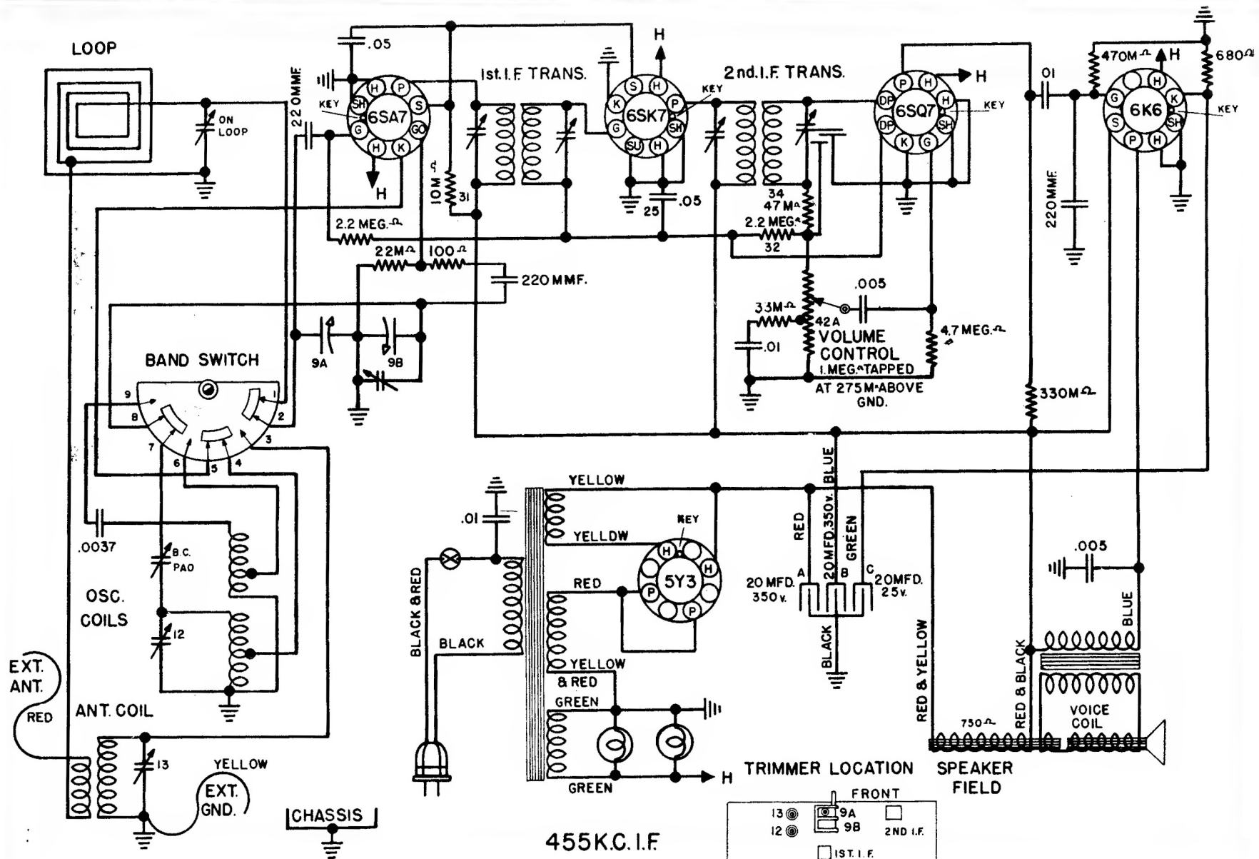
WIRING DIAGRAM — MODEL 53TF
