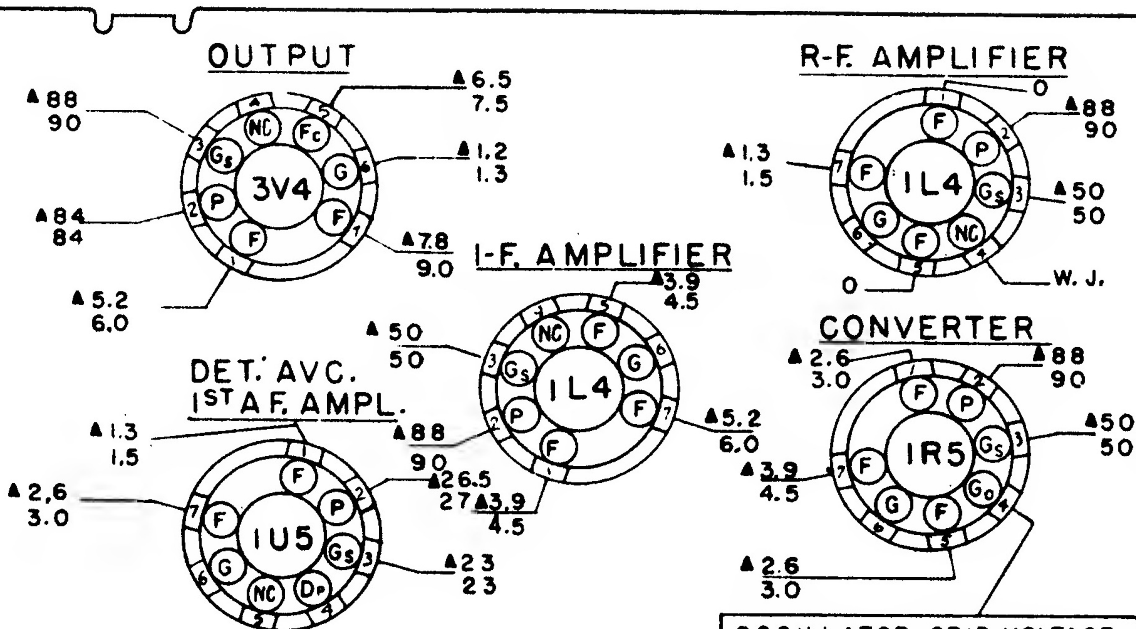
SOCKET VOLTAGE CHART
