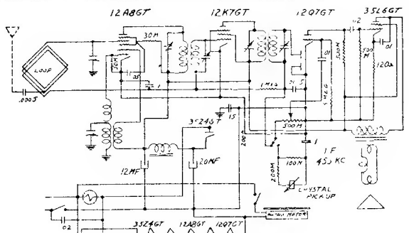
Detrola Model 2741
