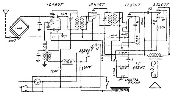
MODEL 2742—A.C.-D.C.—PHONOGRAPH
