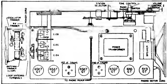
Tube Layout
