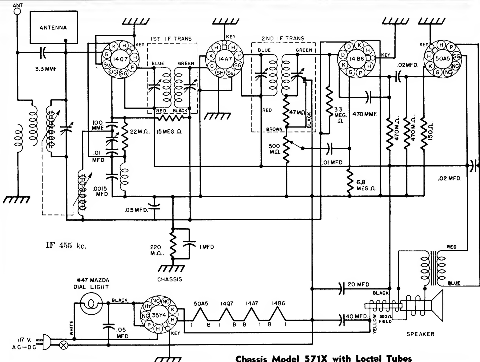
Chassis Model 571X with Loctal Tubes
