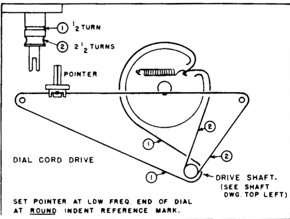
DIAL CORD DRIVE — FOR CHASSIS 120032B
