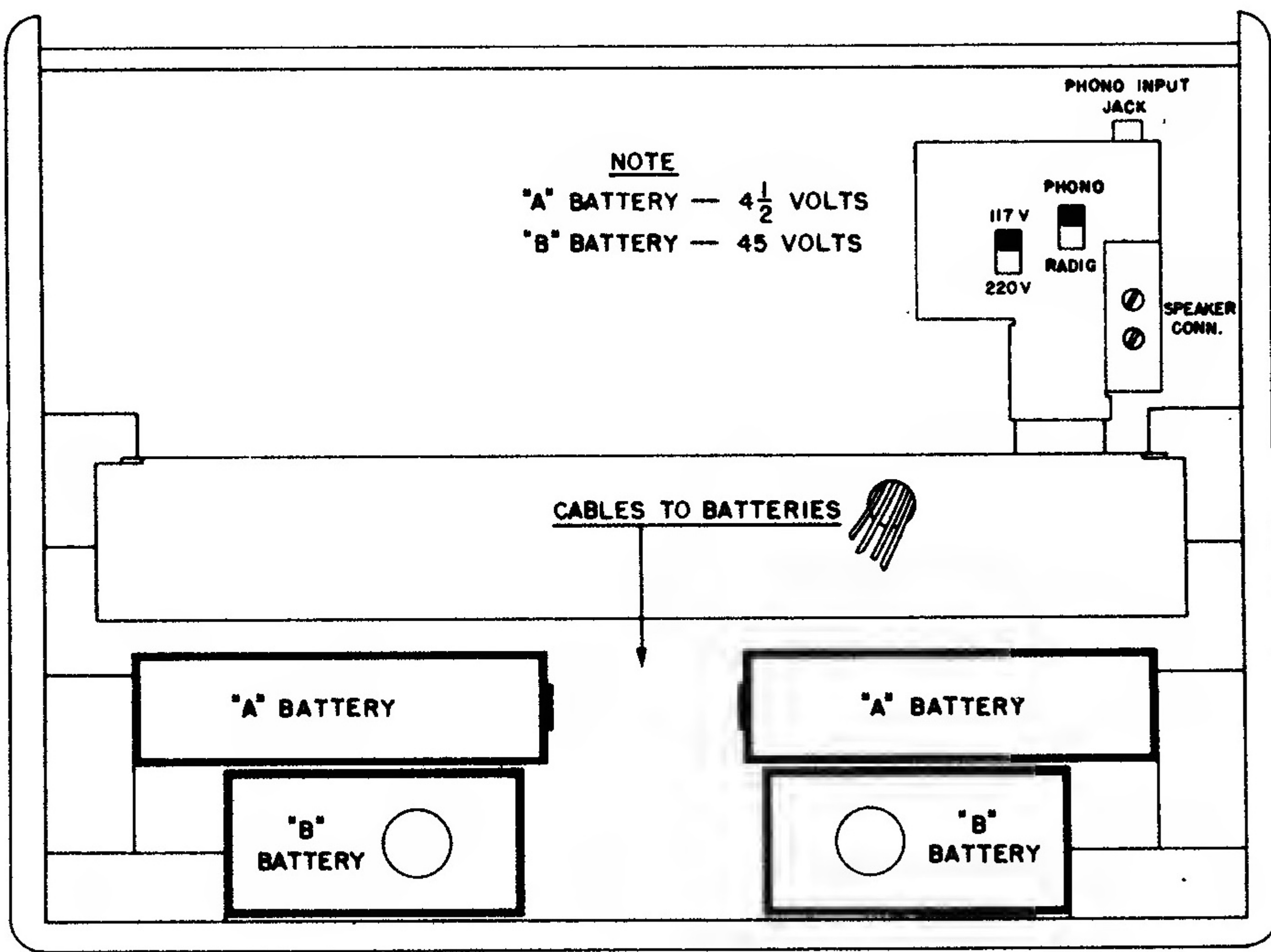
BATTERY LAYOUT P130
