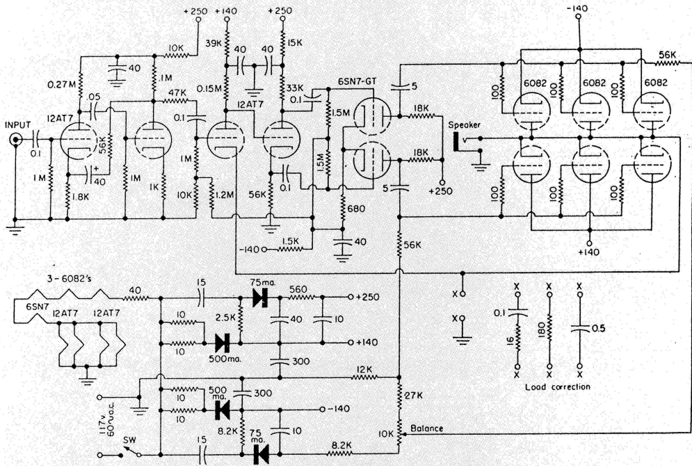
Futterman OTL
