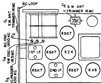
TRIMMER AND TUBE LOCATION DIAGRAM
