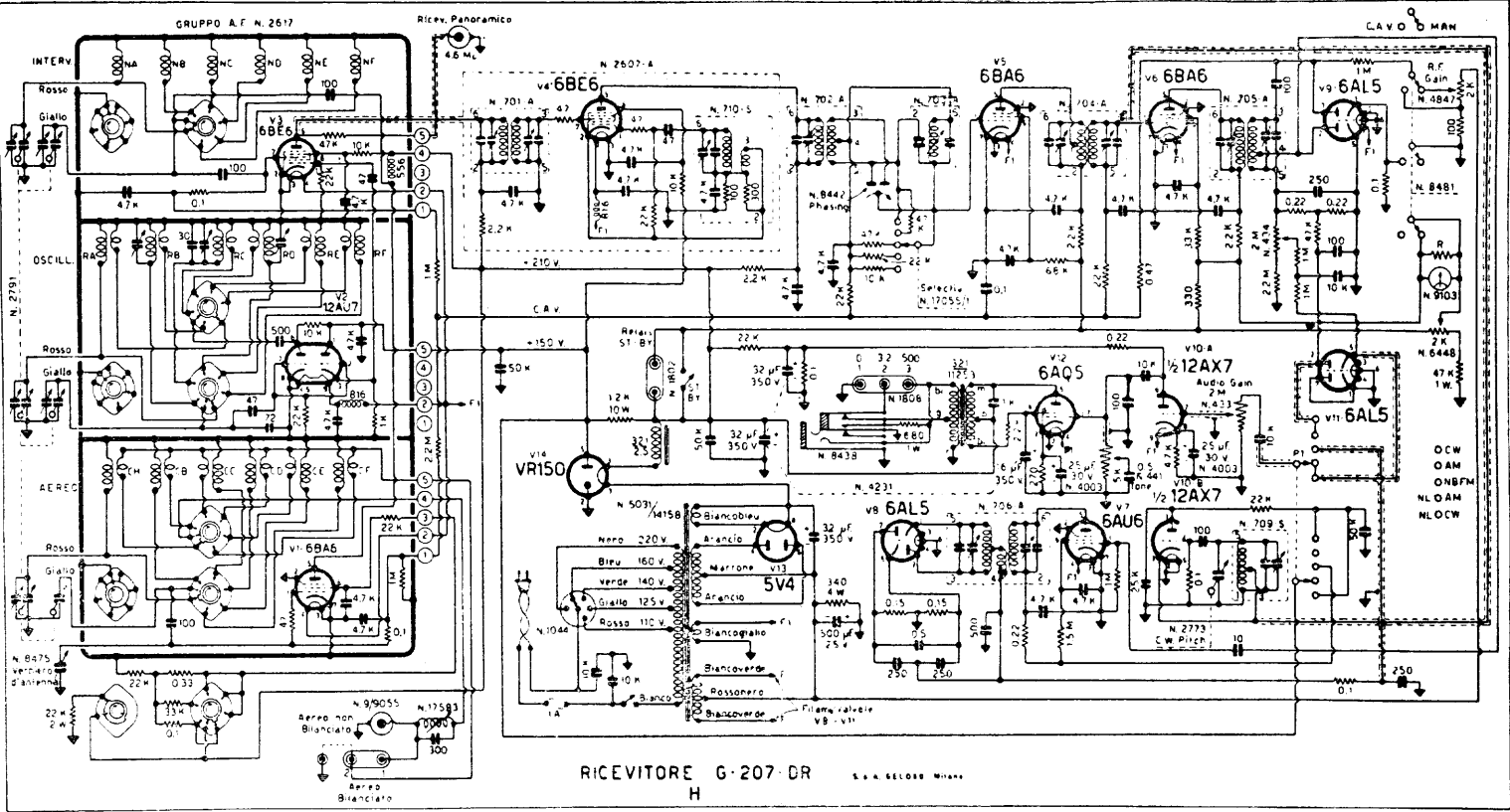
GELOSO S.A. - Mod. Super G 207/DR
