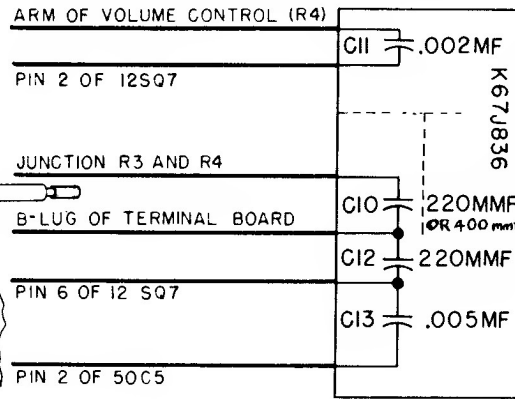
Capacitor Unit C10, 11, 12 and C13
