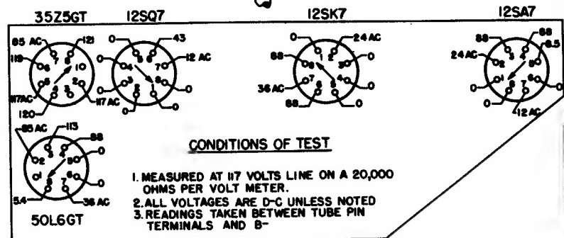
VIEWED FROM BOTTOM OF CHASSIS
