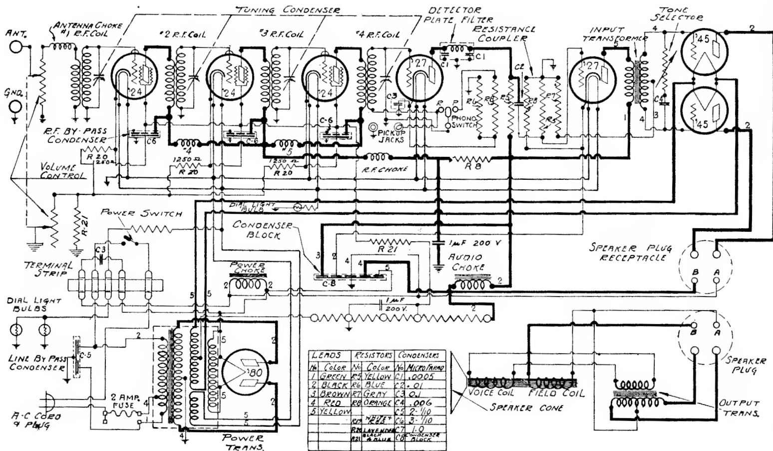
Circuit Diagram of Chassis with Serial Numbers Between 29100A and 6200A; and 1700B and 1946B.
