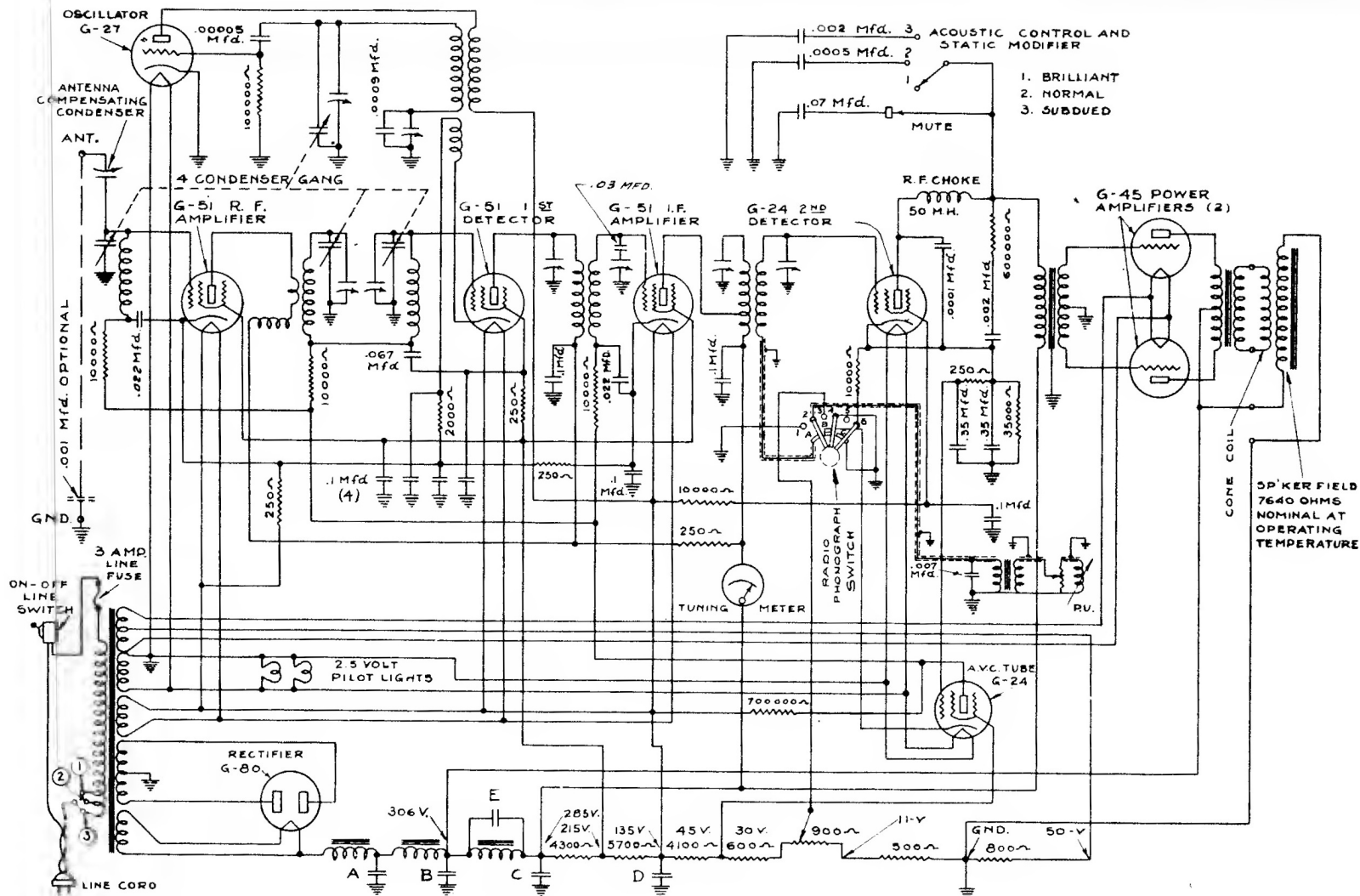
SCHEMATIC DIAGRAM OF MAJESTIC SCREEN GRID SUPERHETERODYNE AUTOMATIC VOLUME CONTROL RECEIVER AND ELECTRIC PHONOGRAPH COMBINATION MODEL 160 CHASSIS 115 AND 220 VOLTS, 25 - 40 AND 50 - 60 CYCLES.
