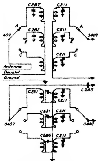
Brain Schematic for Sets Incorporating Long Wave or "E" Band. (125-350 KC.)
