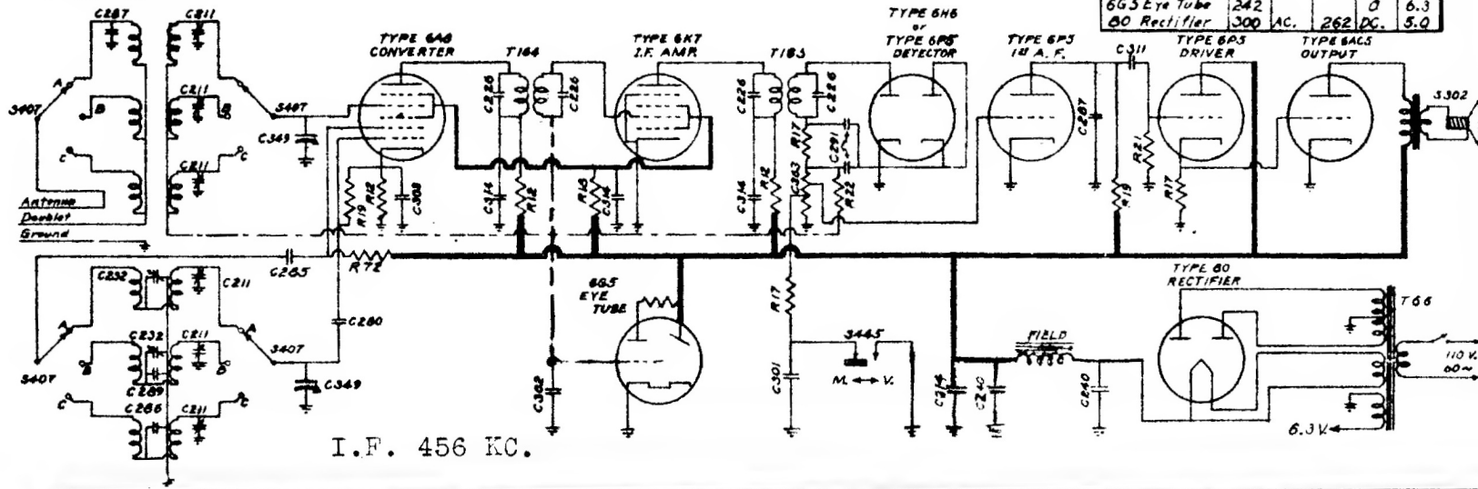
Standard Brain Below Incorporates Police Band. 1.7-5.5 MG.
