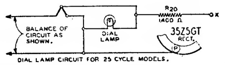
DIAL LAMP CIRCUIT FOR 25 CYCLE MODELS.
