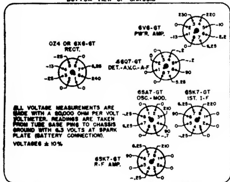
BOTTOM VIEW OF CHASSIS
