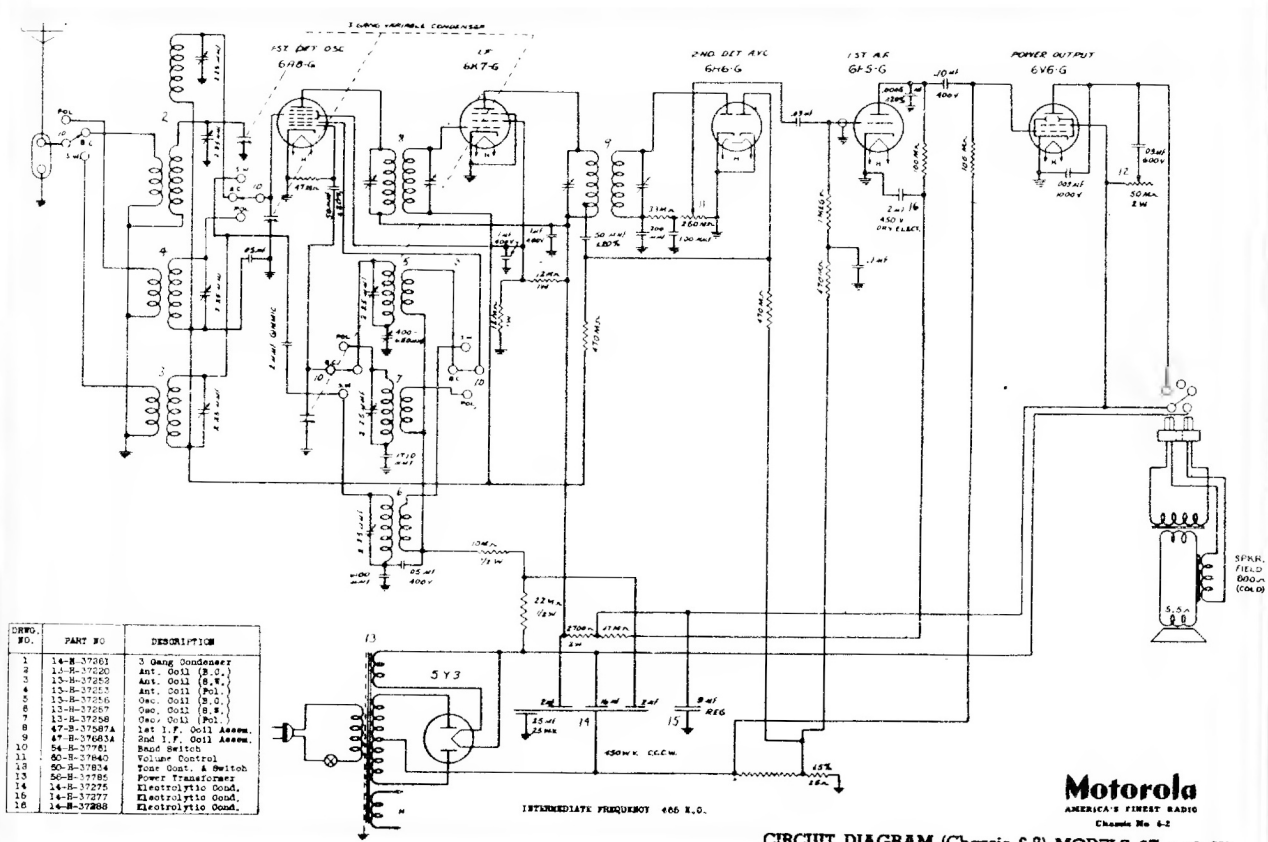
CIRCUIT DIAGRAM (Chassis 6-2) MODELS 6T and 6Y
