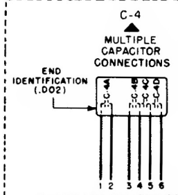
DIAGRAM OF CHASSIS USING MULTIPLE CERAMIC CAPACITOR
