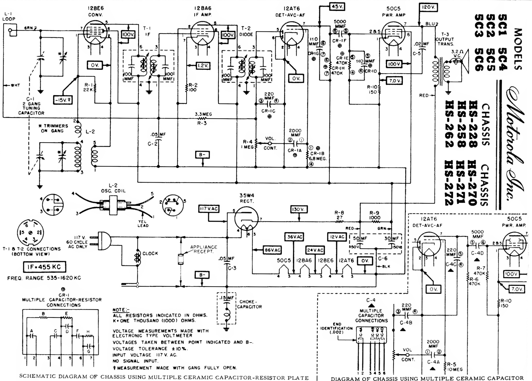
DIAGRAM OF CHASSIS USING MULTIPLE CERAMIC CAPACITOR
