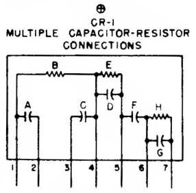
SCHEMATIC DIAGRAM OF CHASSIS USING MULTIPLE CERAMIC CAPACITOR-RESISTOR PLATE
