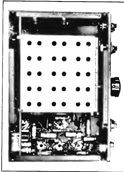
BOTTOM VIEW The coil assembly is shown midway between the 1.3-2.8 mc. and 2.7-6.4 mc. ranges.
