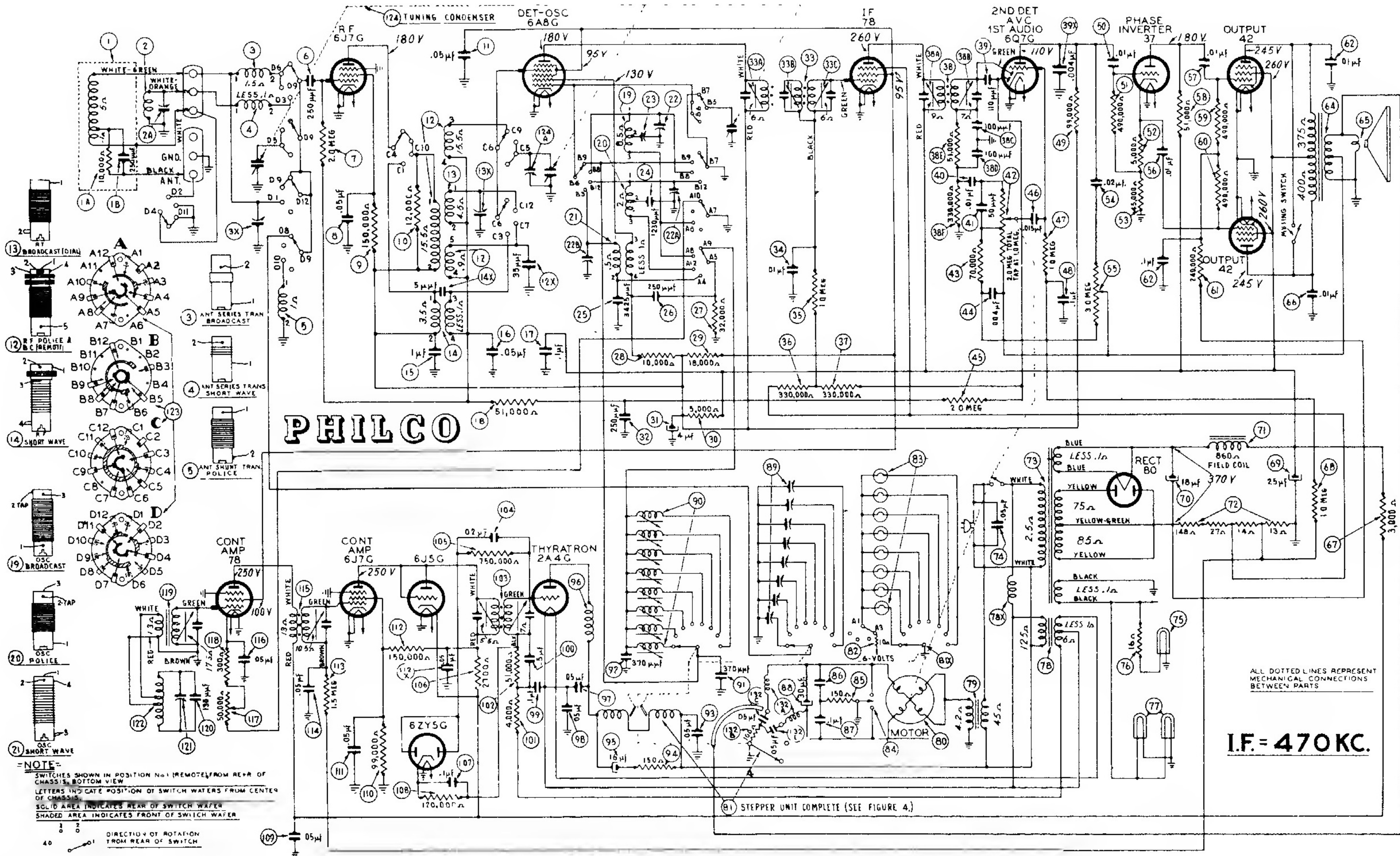
SCHEMATIC DIAGRAM MODEL 40-216
