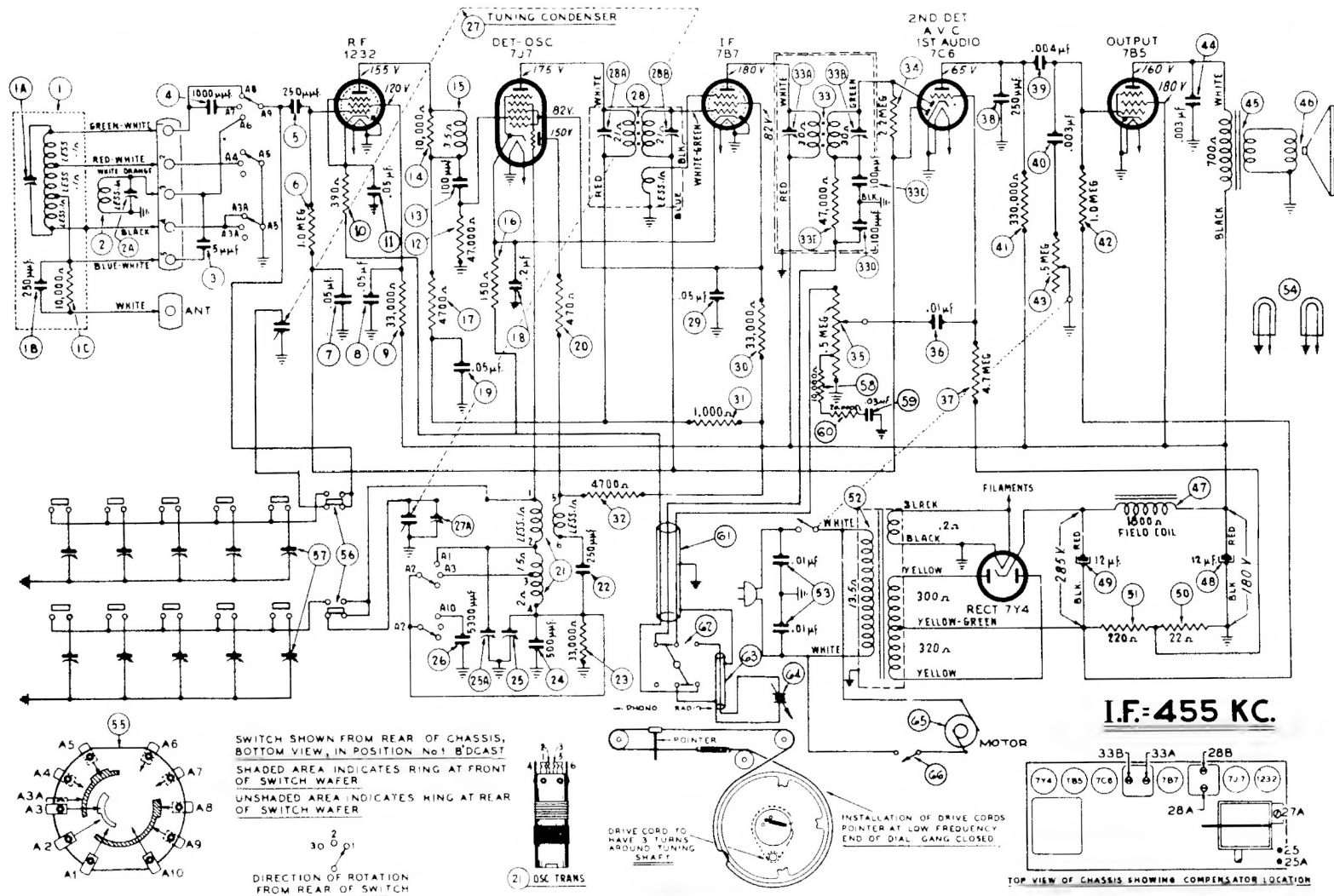
SCHEMATIC DIAGRAM MODEL 40-507
