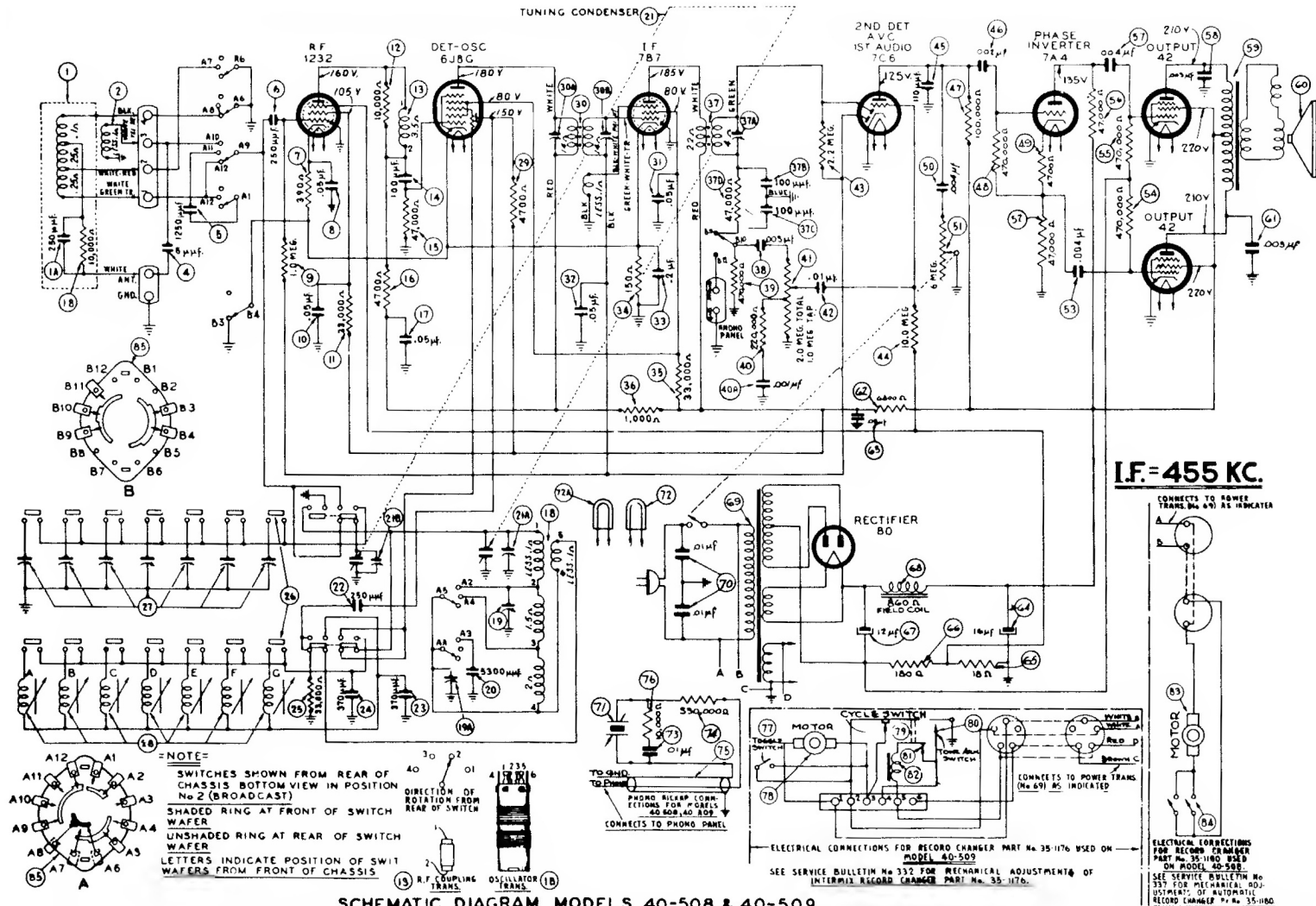
SCHEMATIC DIAGRAM MODELS 40-508 & 40-509
