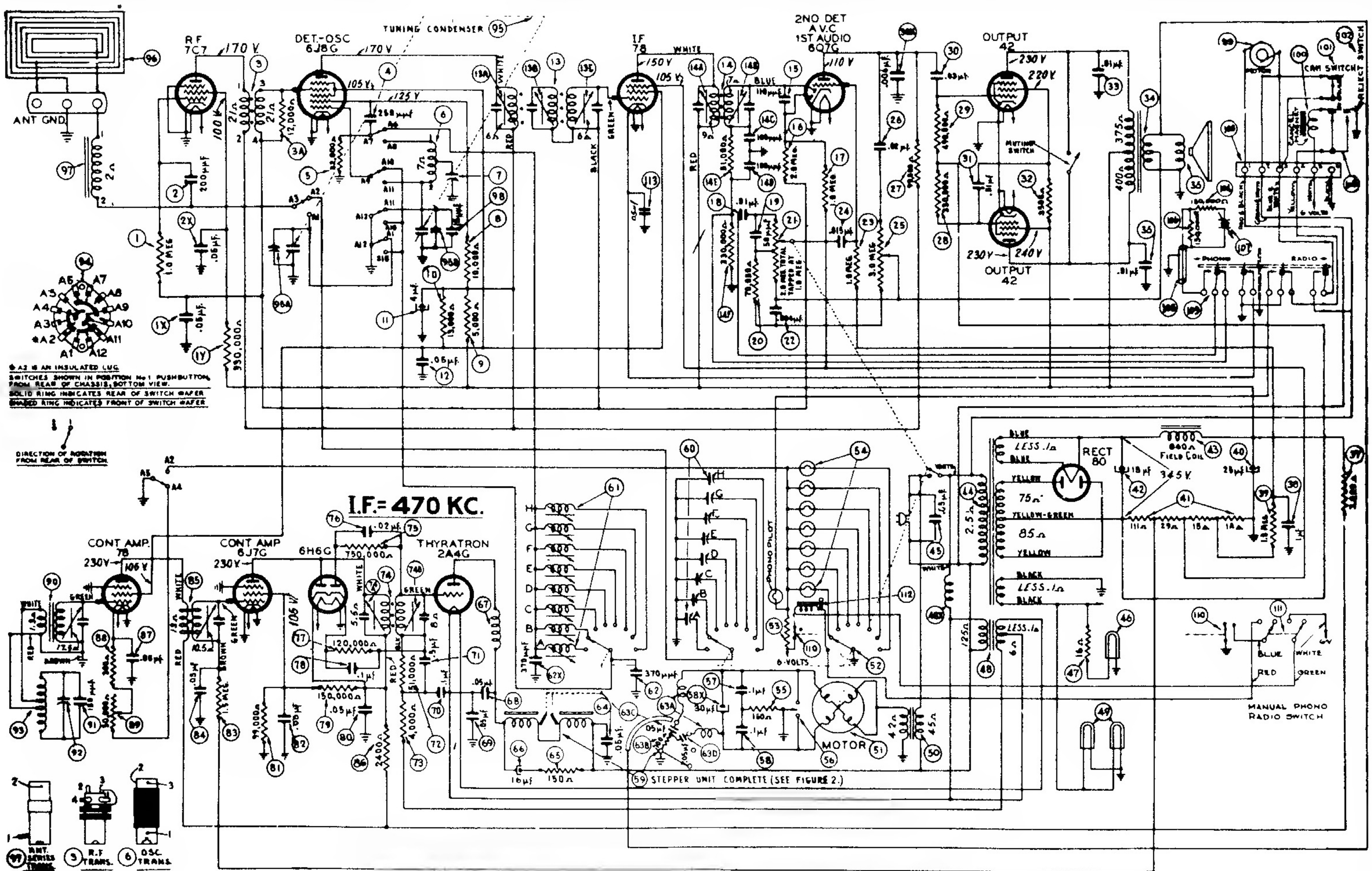
SCHMATIC DIAGRAM MODEL 40-510
