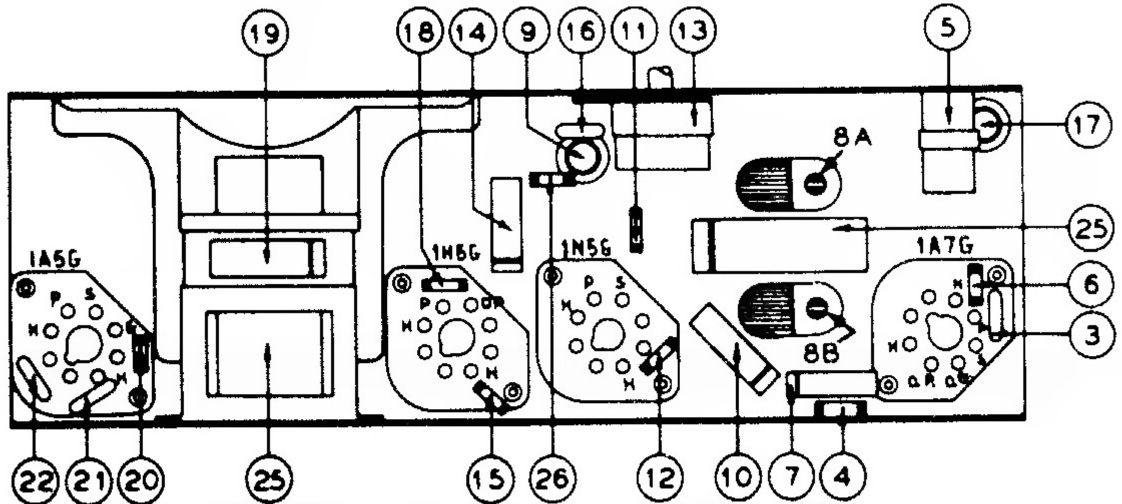
PART LOCATIONS, UNDERSIDE OF CHASSIS, MODEL 40-81
