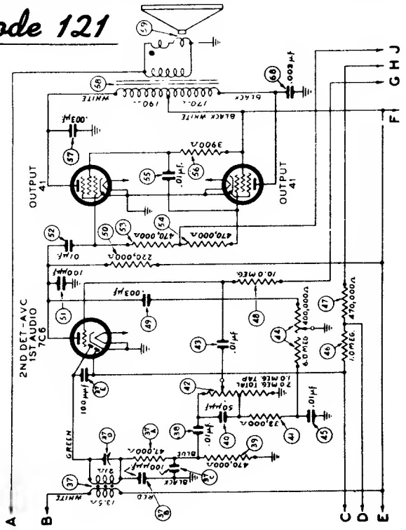
2ND DETECTOR AND AUDIO CIRCUIT MODEL 41-250
