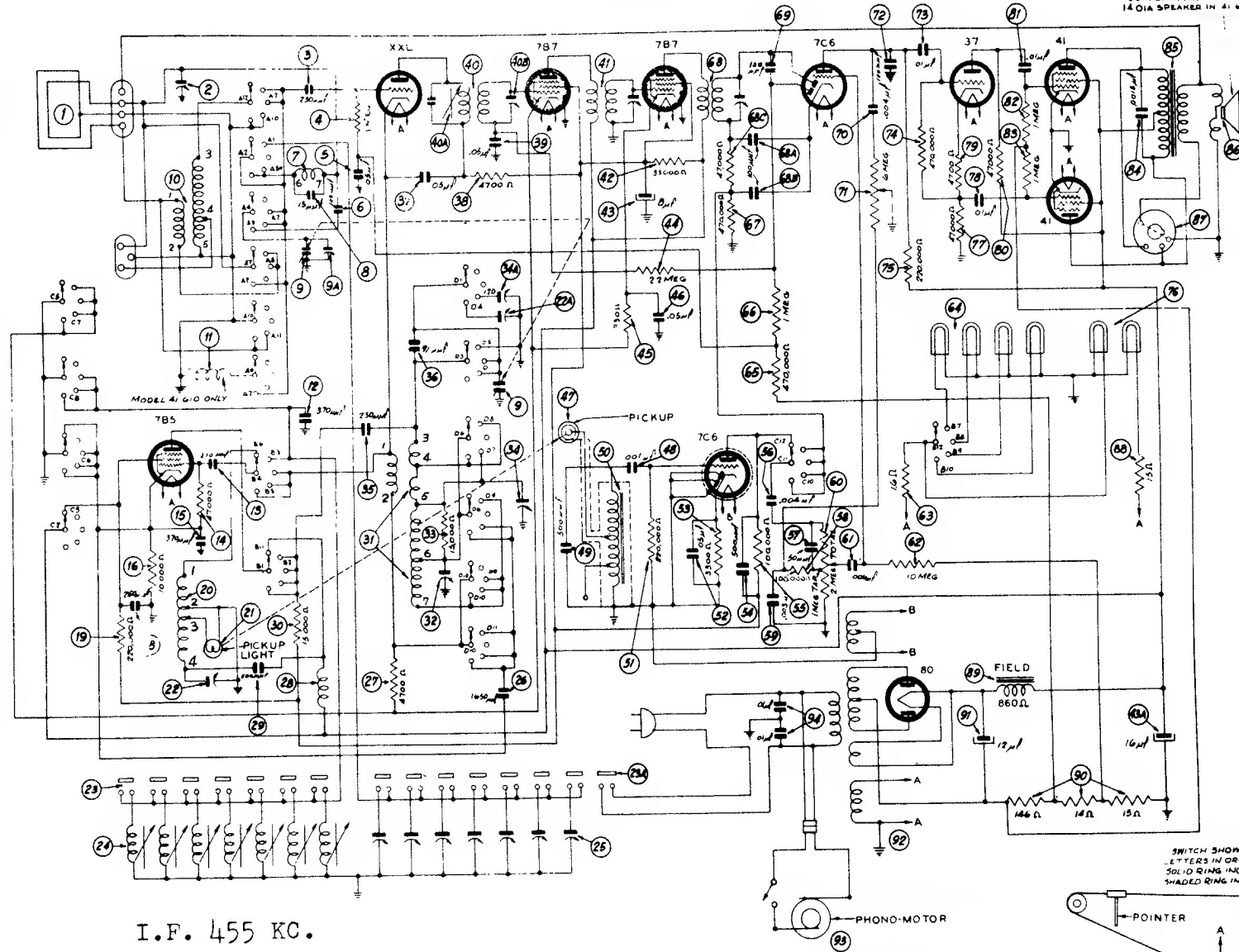
SCHEMATIC DIAGRAM—MODELS 41-610 41-611. CODE 121
