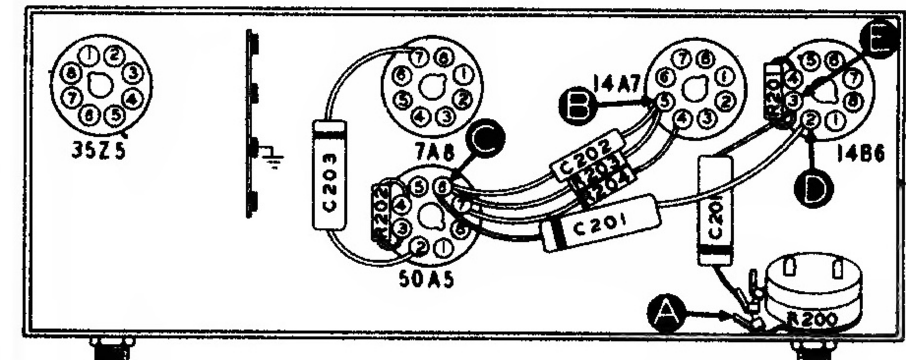
FIGURE 2. BOTTOM VIEW, SHOWING SECTION 2 TEST POINTS
