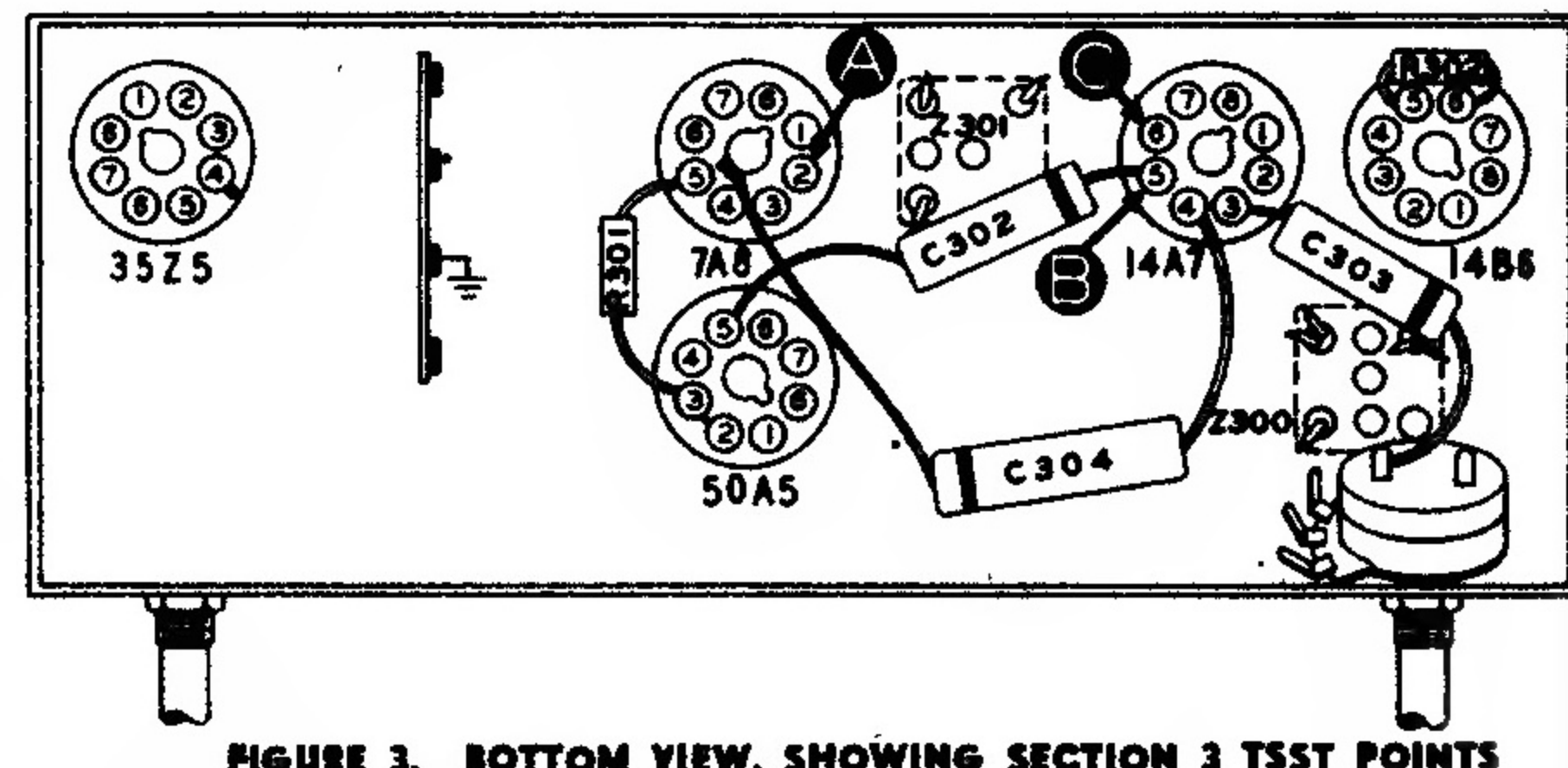
FIGURE 3. BOTTOM VIEW, SHOWING SECTION 3 TEST POINTS
