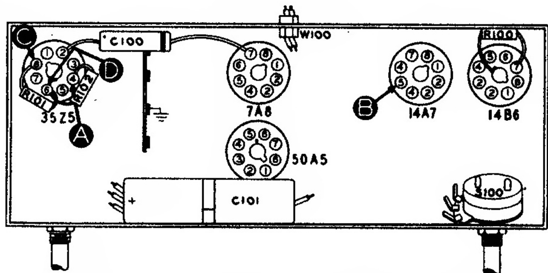
FIGURE 1. BOTTOM VIEW, SHOWING SECTION 1 TEST POINTS
