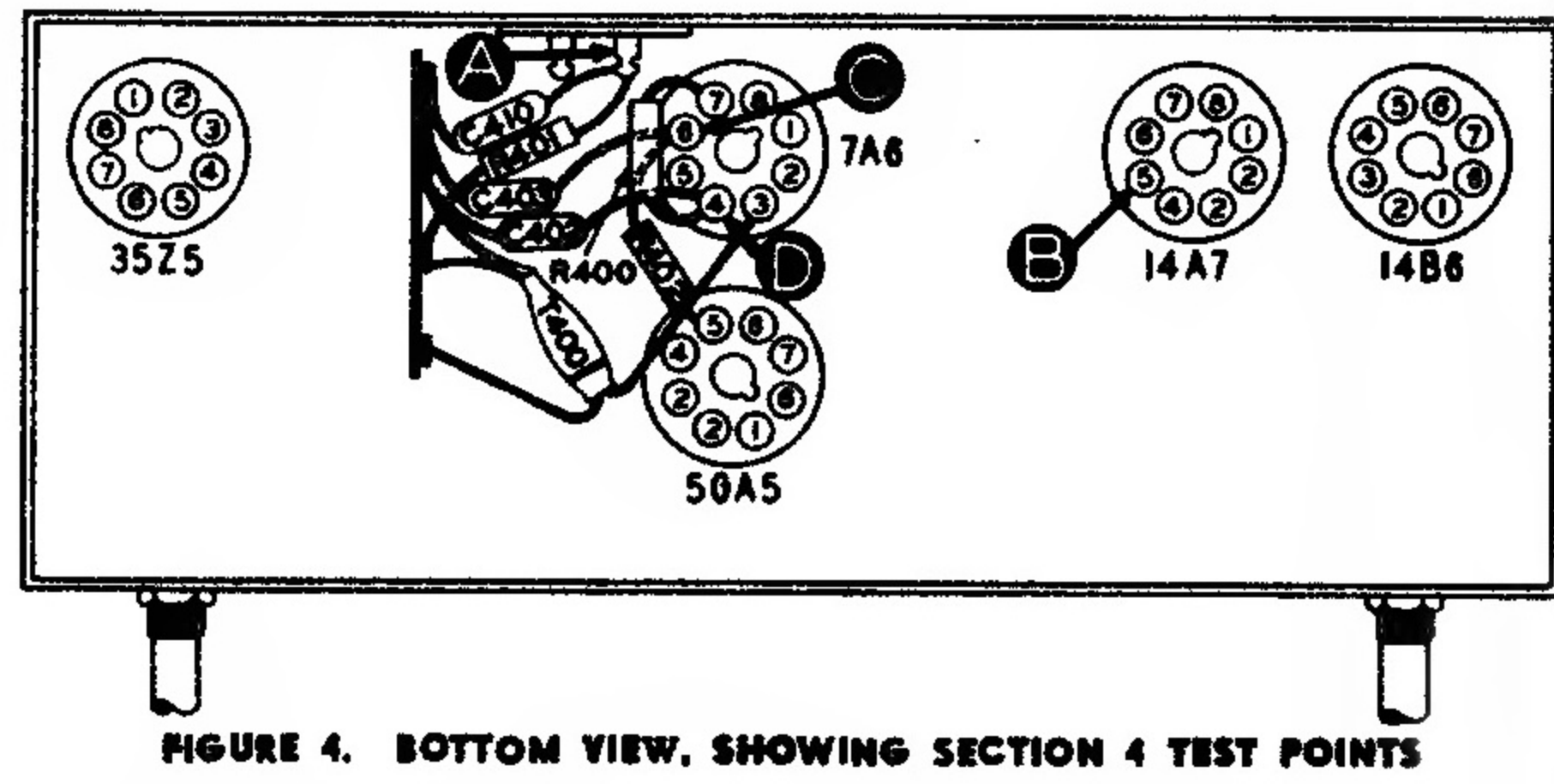
FIGURE 4. BOTTOM VIEW, SHOWING SECTION 4 TEST POINTS
