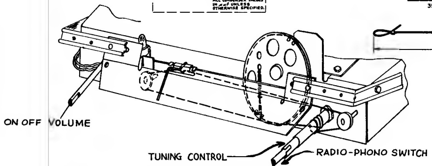
Drive-Cord Installation Details
