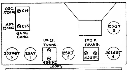
TUBE & TRIMMER LOCATIONS
