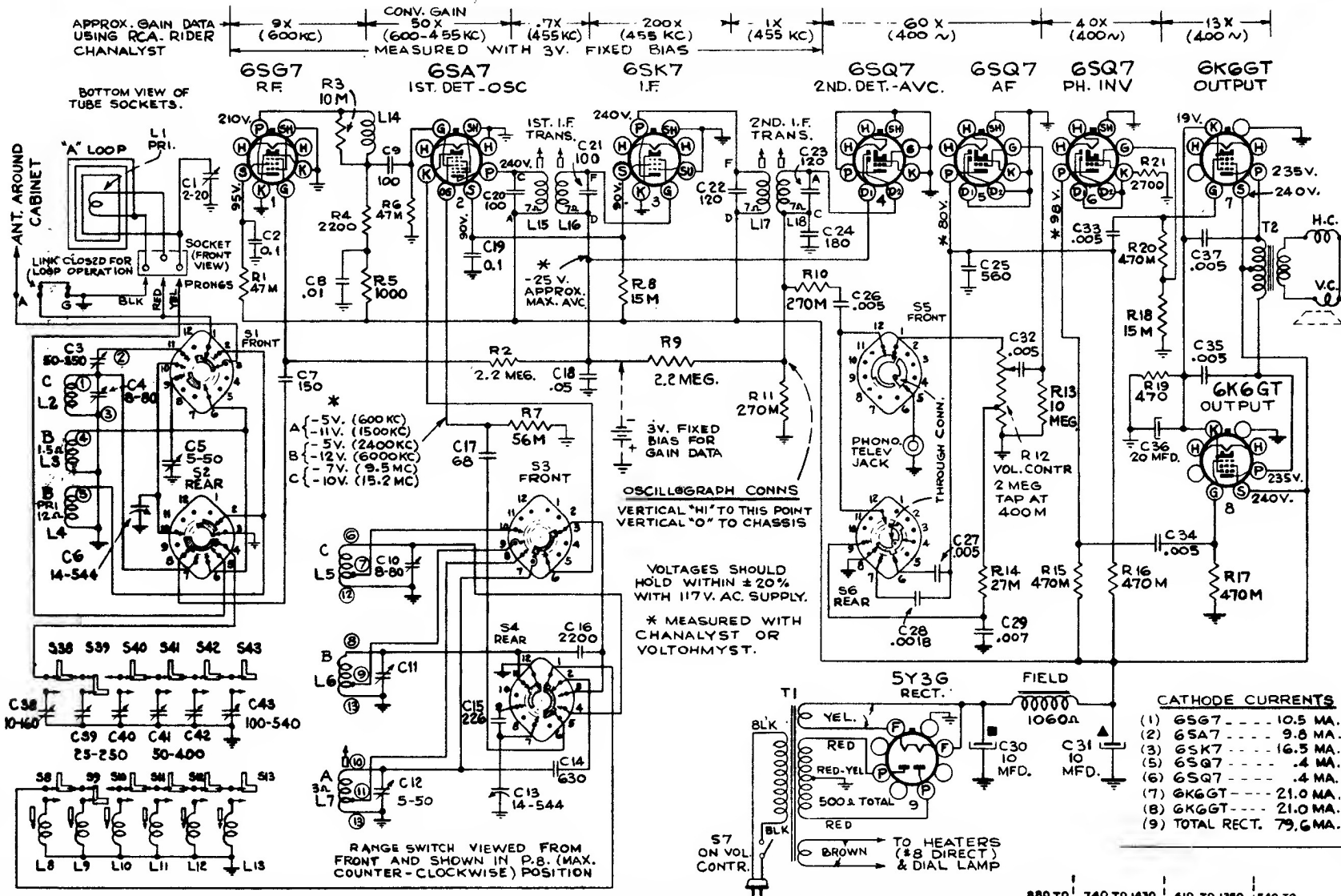
Model 29K Schematic Diagram
