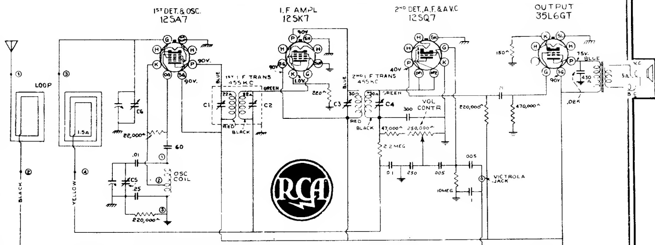
LOOP CONNECTIONS
