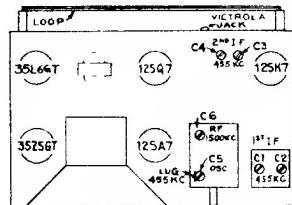
TUBE AND TRIMMER LOCATIONS
