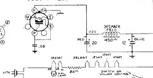
35Z5GT - RECT.
