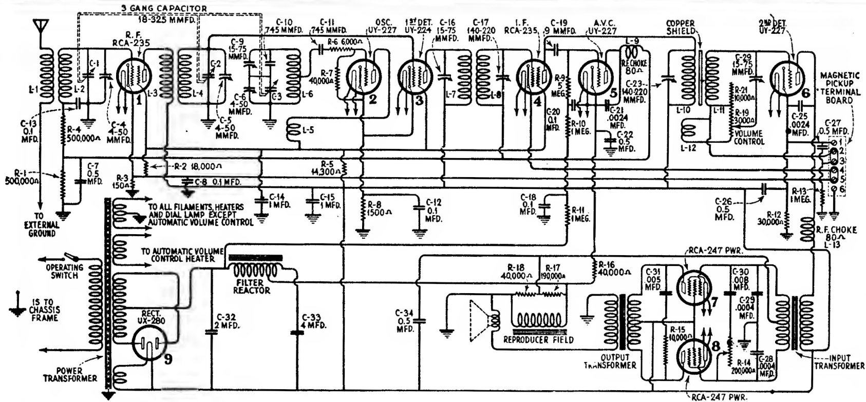
R.C.A. Schematic Circuit Diagram of Model R-11
