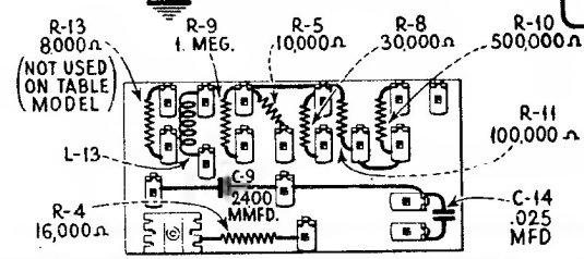
RESISTOR BOARD CONNECTIONS
