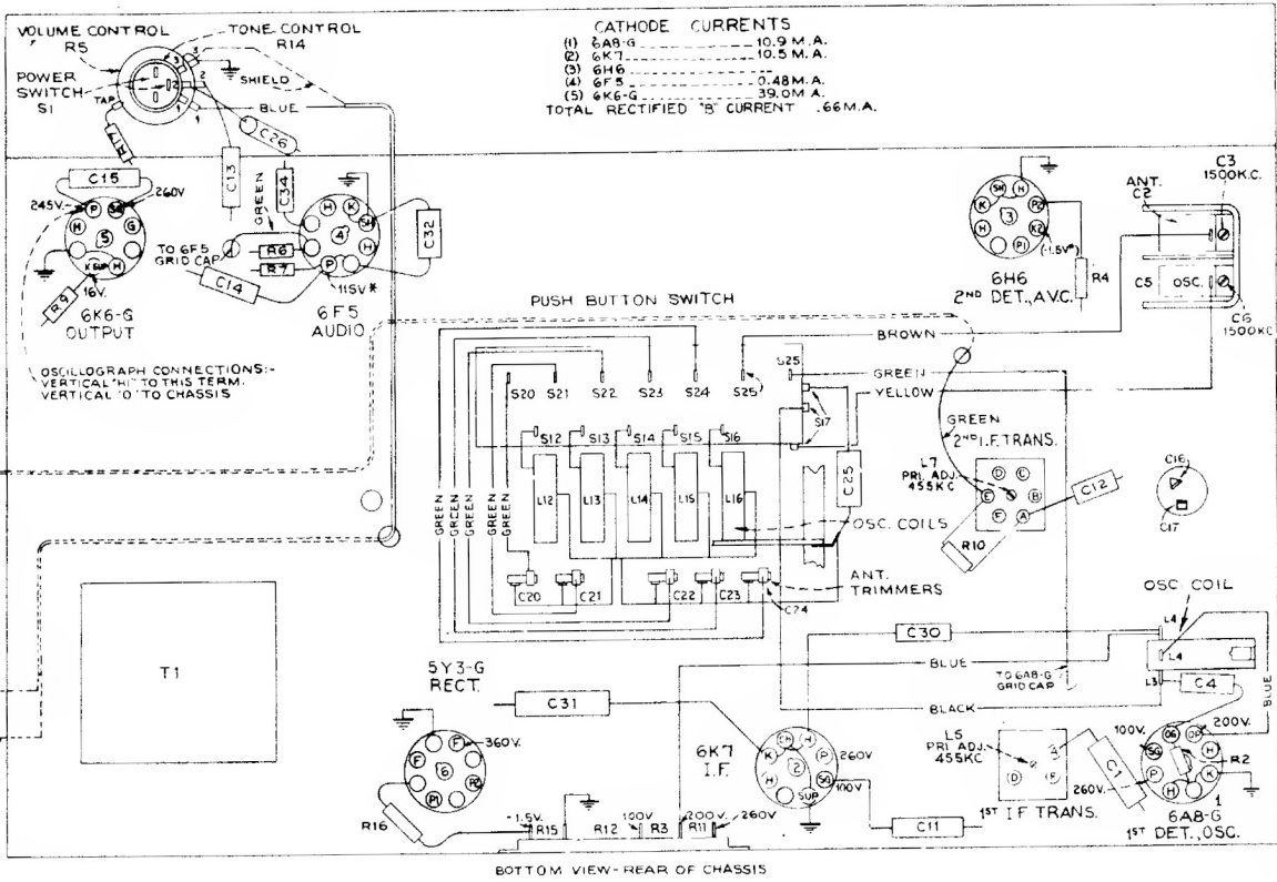
BOTTOM VIEW - REAR OF CHASSIS
