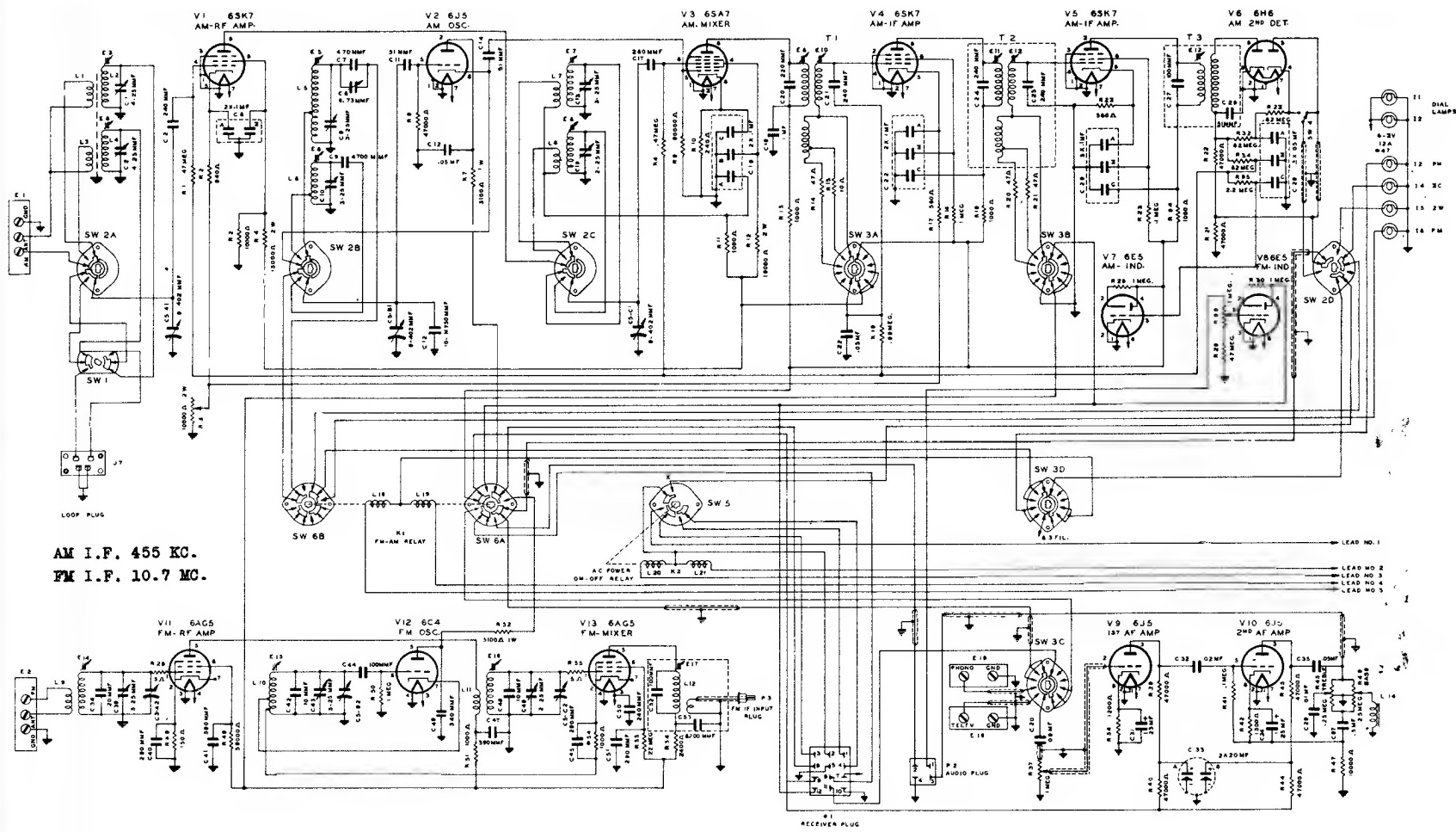
Revised Schematic Diagram Model 800-B Receiver Chassis
