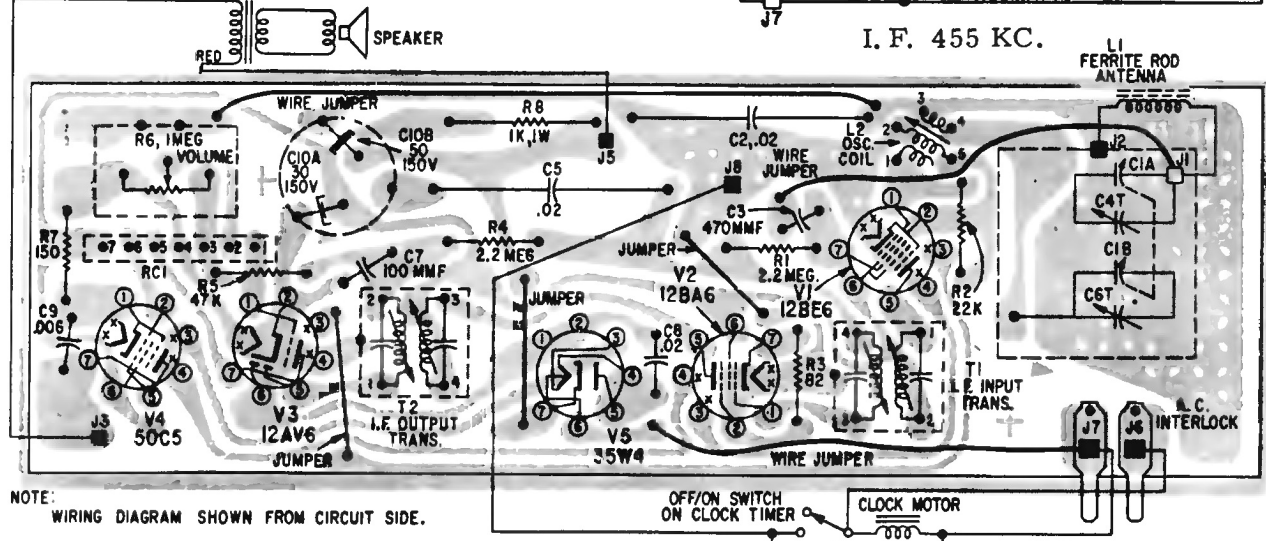
Circuit Board Wiring Diagram, 84-12074-0
