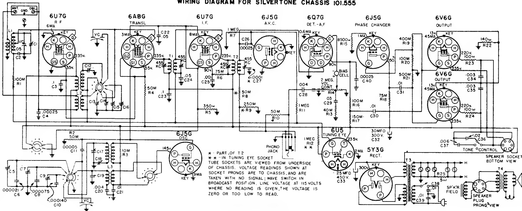
WIRING DIAGRAM FOR SILVERTONE CHASSIS 101.555
