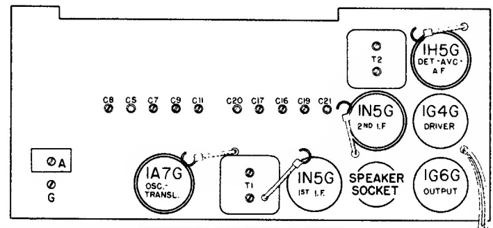
LOCATIONS OF PARTS ON TOP OF CHASSIS.
