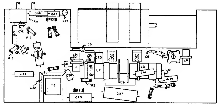
LOCATIONS OF PARTS UNDER CHASSIS
