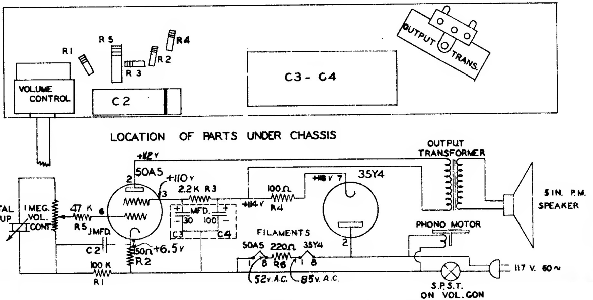
AMPLIFIER SCHEMATIC DIAGRAM 431.199
