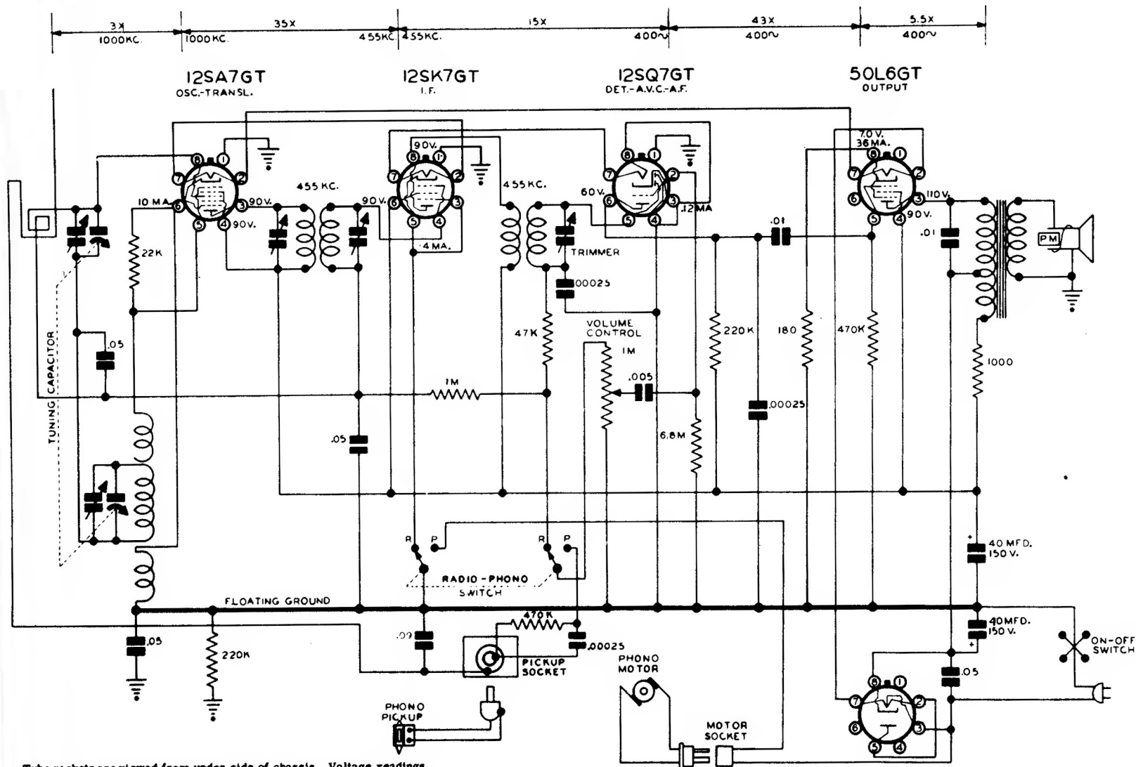
SCHMATIC DIAGRAM FOR 135.244
