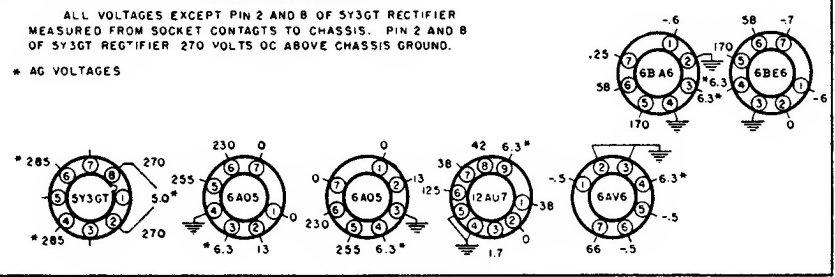
VOLTAGE TABLE (180° BOTTOM VIEW OF CHASSIS)
